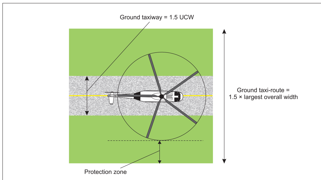
Figure 3-2. Ground taxi-route
